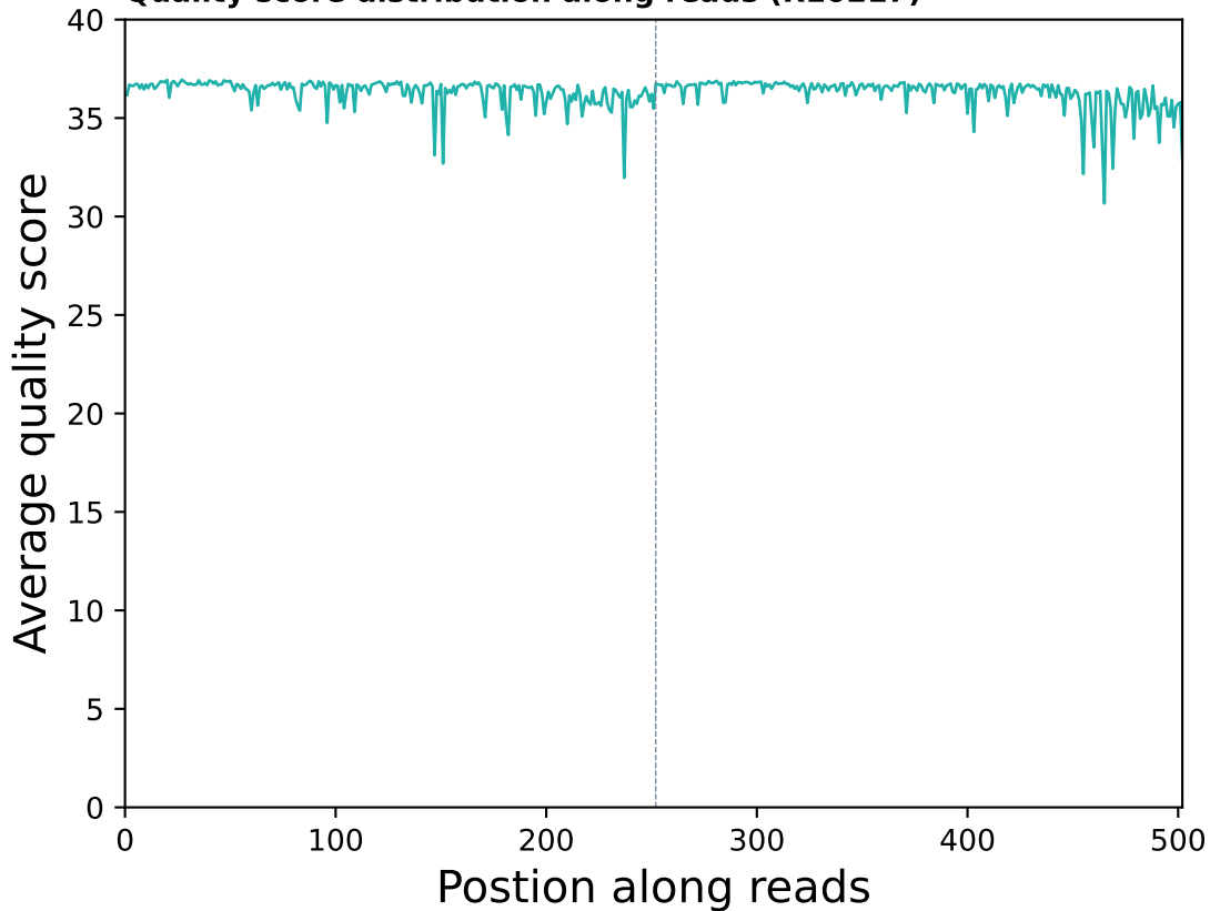
Quality score distribution along reads (R10217)
